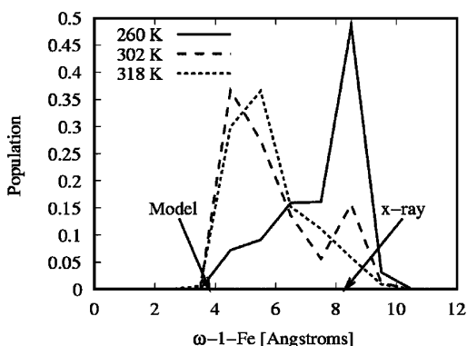
Figure 3. Population distribution of conformations of the P450 BM-3/NPG complex as a function of \omega-1 -Fe distance at temperature 260 K (—), 302 K (---), and 318 K (···). The arrows indicate the values of the \omega-1 -Fe distance in the X-ray crystal structure (1j pz) and the conformation modeled by Jovanovic et al. At 260 K, most of the population is concentrated in the peak corresponding to the distal state. At 302 K, population peaks corresponding to both proximal and distal states are seen. At 318 K, the proximal state is the most populated.
