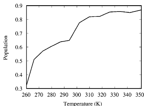
Figure 4. Population as a function of temperature p(T) corresponding to the conformations in which ligand is proximal to the heme iron (obtained by integration of the population distribution from Figure 2 along the \omega-1 -Fe distance coordinate between 0 and 6.5 Å). The proximal state population increases monotonically with temperature indicating that the proximal state is stabilized by conformational entropy at temperatures greater than at least 268 K. This is borne out by the expression for the conformational entropy difference between the proximal and the distal states: \Delta S = k \ln[p/(1-p)] + \{kT/[p(1-p)]\} \partial p/\partial T , where the second term is positive and the first term is positive for T > 268 K ( p(T) > 1/2 ).
