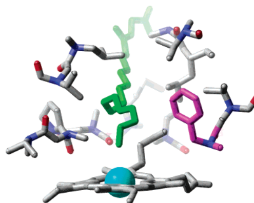
Figure 6. Active site of the P450 BM-3/NPG complex in a representative proximal free ligand conformation. Note that in this conformation not only has the side chain Phe87 (shown in magenta) changed its rotameric state to allow NPG (shown in green) to approach the heme iron (shown in blue), but also Phe87 is oriented so as to give NPG the ability to move more freely (as compared to the proximal state conformation predicted by Jovanovic et al.) to and away from the heme.
